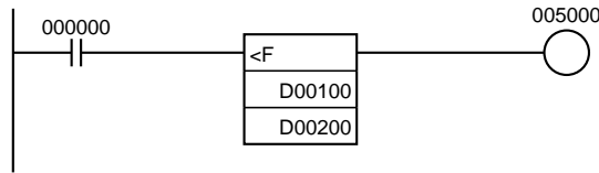
FLOATING LESS THAN Comparison (<F)
